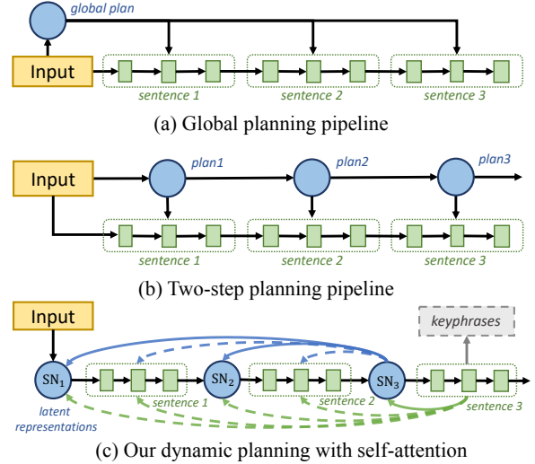
Figure 2: Comparison of different content planning. For (c), the blue arrow denotes the attention flows for latent representations and the green one for target words. The attention of tokens within the same sentence is omitted. We highlight the attention flows related to the content planning with solid lines for sentence 3. Best viewed in color.
